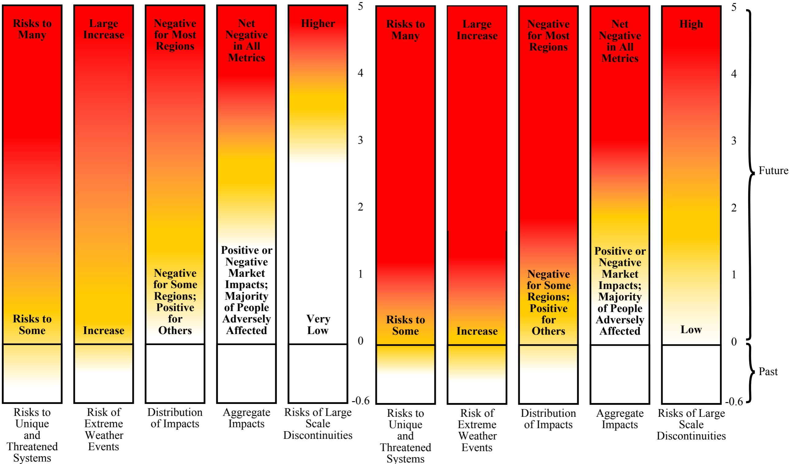
Proposed AR4 (2007) Reasons For Concern
